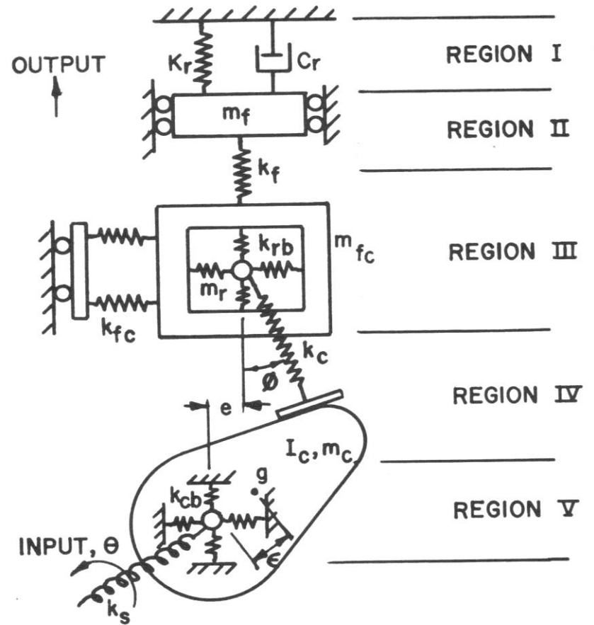
Figure 1-3. A Possible System Model.
