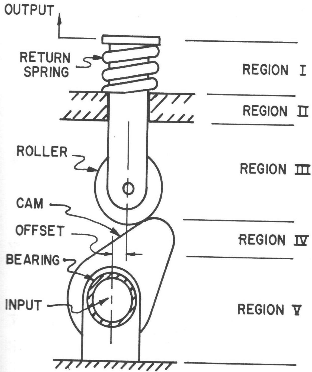
Figure 1-2. A Typical Cam System.
