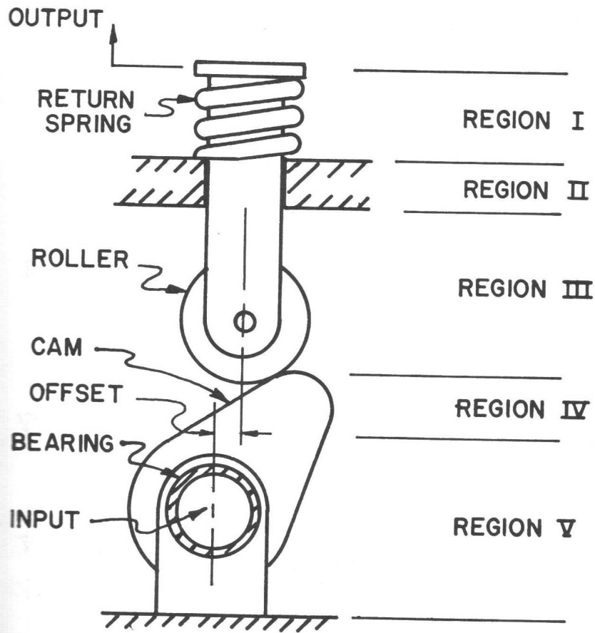
Figure 1-2. A Typical Cam System.
